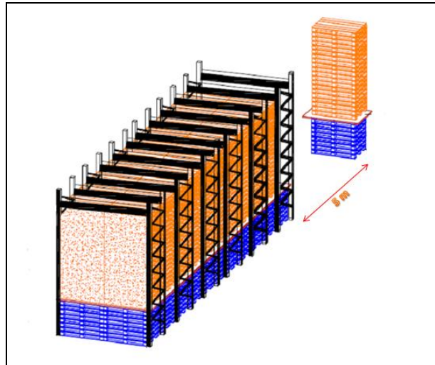
Figure 11. Location of fire target 5m downstream of the mock-up
