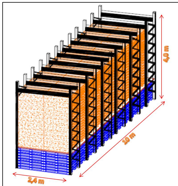
Figure 5. Mock-up dimensions
